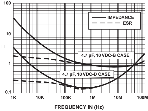
TYPICAL CURVES AT + 25 °C, IMPEDANCE AND ESR VS. FREQUENCY
