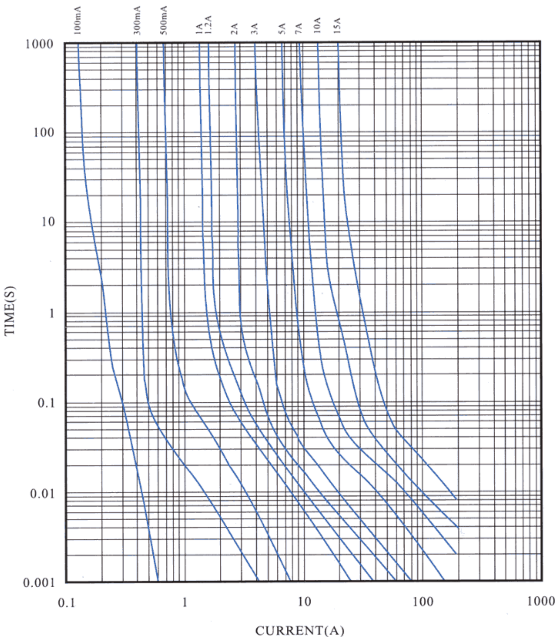
I-T CHARACTERISTICS CURVE
