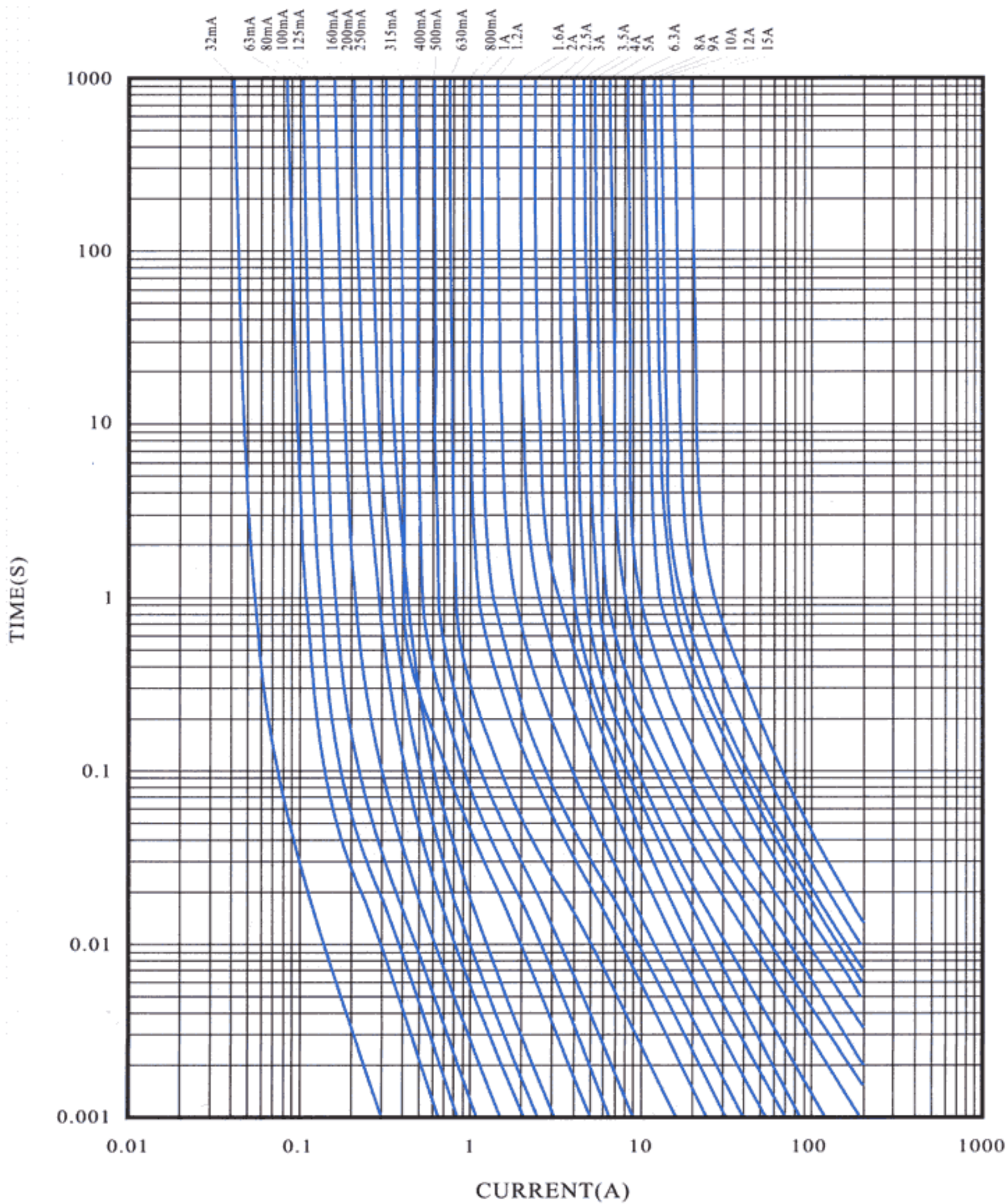
I-T CHARACTERISTICS CURVE
