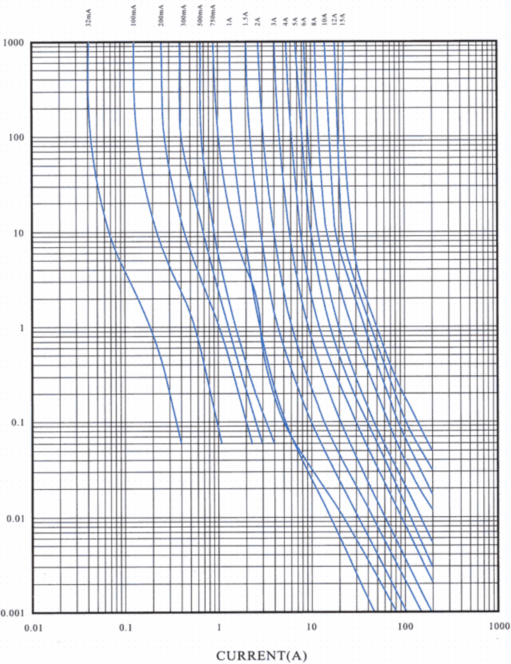
I-T CHARACTERISTICS CURVE
