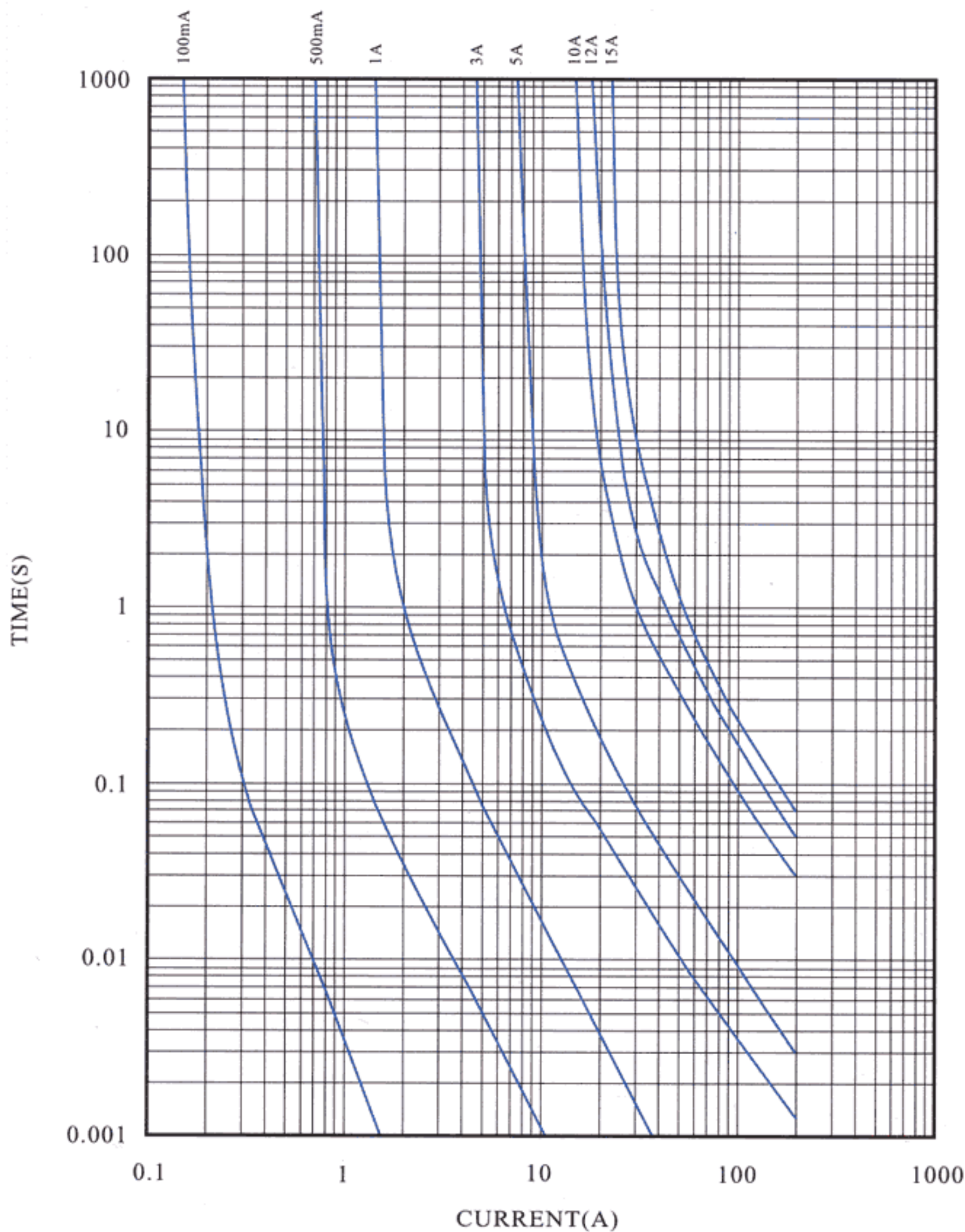
I-T CHARACTERISTICS CURVE
