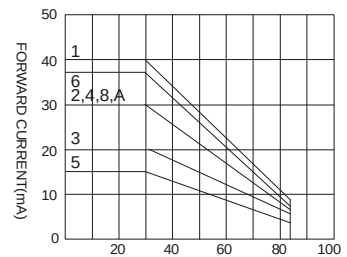
FORWARD CURRENT VS. AMBIENT TEMPERATURE
