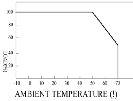
Derating Curve
