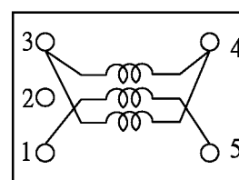
Transformer Fig.4
