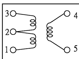
Transformer Fig.2
