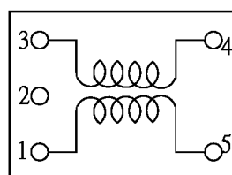
Transformer Fig.3
