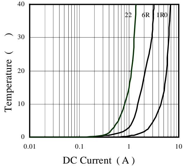
@ DC Current VS. Temp. Rise ( T ) Curve
