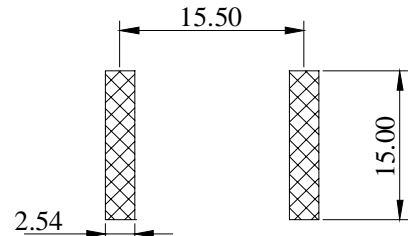
( PCB Pattern )
