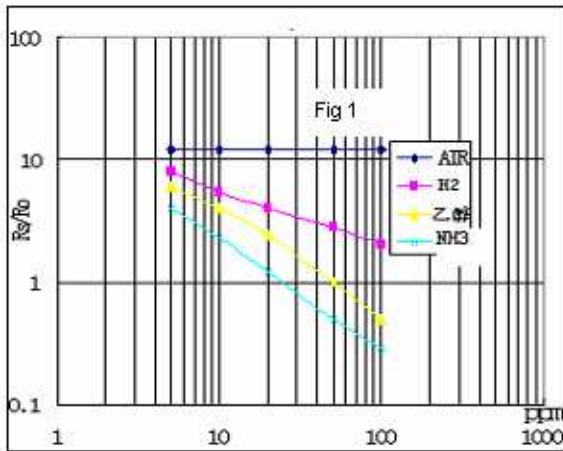
Fig.1 shows the typical sensitivity characteristics of the MQ137, ordinate means resistance ratio of the sensor ( R_s/R_o ), abscissa is concentration of gases. R_s means resistance in different gases, R_o means resistance of sensor in 50ppm ethanol. All test are under standard test conditions.
