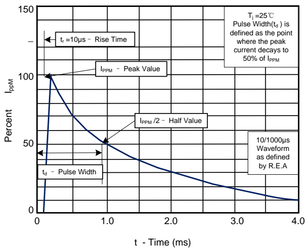
Figure 3. Pulse Waveform
