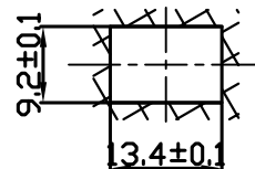
Panel Installation Thickness 1 ~ 4mm
