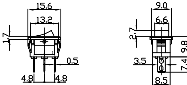
YSR-10-12 (B) On-On (Unilluminate)
