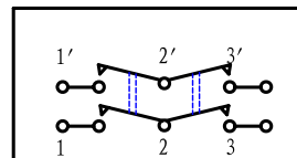
On-Off-On (Unilluminate)
