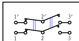
On-On (Unilluminate)
