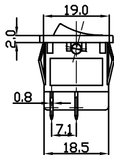
On-On (Unilluminate)
