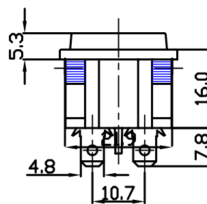
On-Off-On (Unilluminate)
