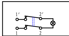
On-Off (Illuminate)
