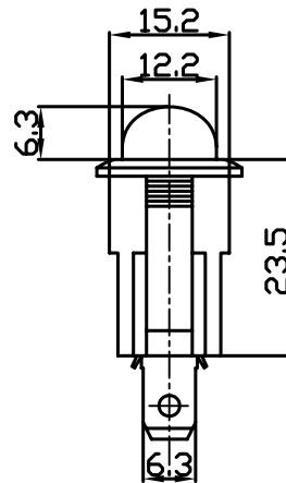
YSR-8-11/N On-Off (Illuminate)
