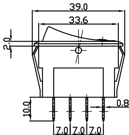
YSR-8-21/N On-Off (Illuminate)
