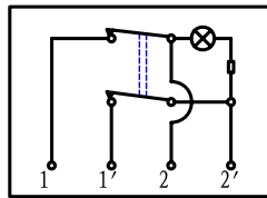
YSR-8-21/N On-Off (Illuminate)
