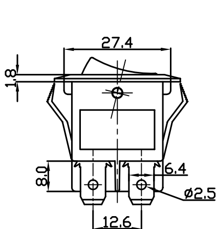
YSR-9-21 (A) /N On-Off (Illuminate)
