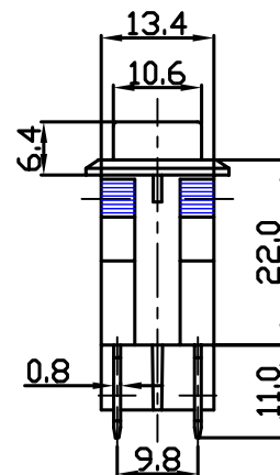
YSR-9-21 (A) On-Off (Unilluminate)
