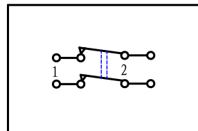
YSR-9-21 (A) On-Off (Unilluminate)
