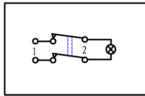
YSR-9-21 (C) /N On-Off (Illuminate)
